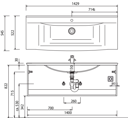
SWM G140
